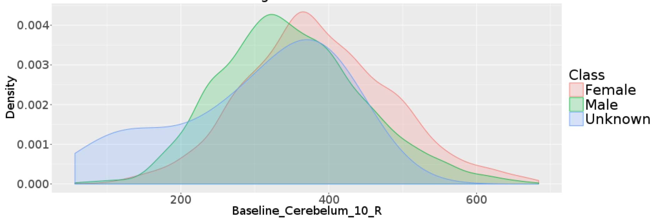
Marginal Distribution
