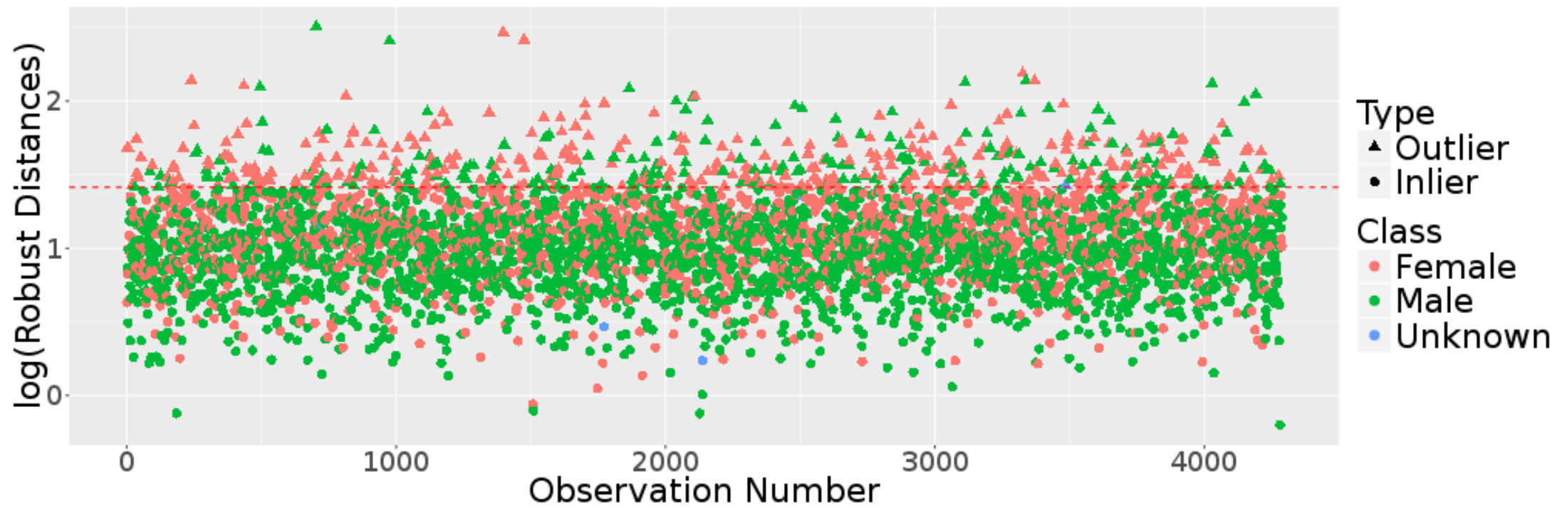
Outlier Plot
