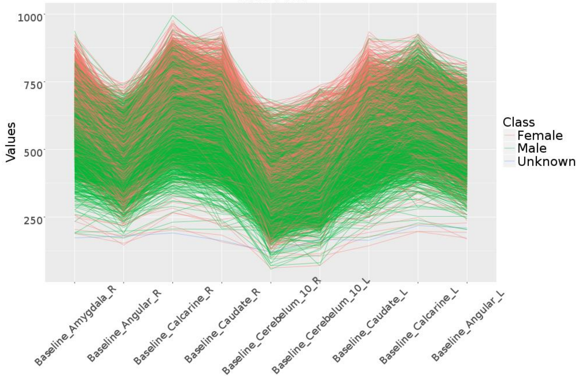
Line Plot
