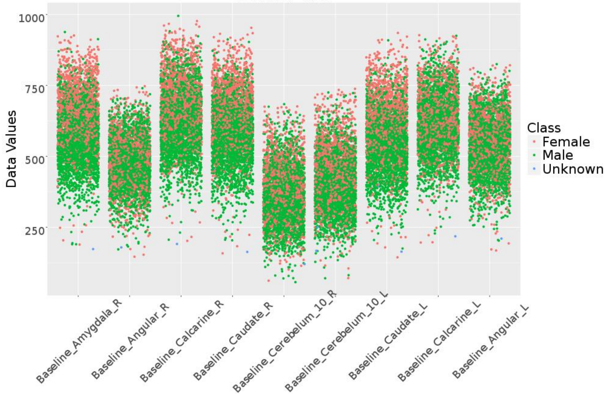
Scatter Plot
