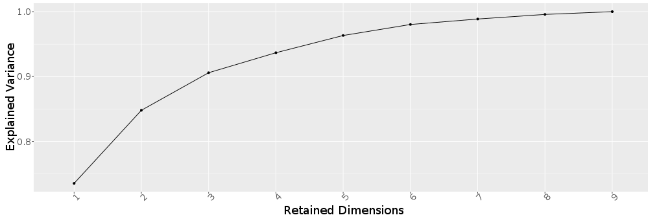
Scree Plot
