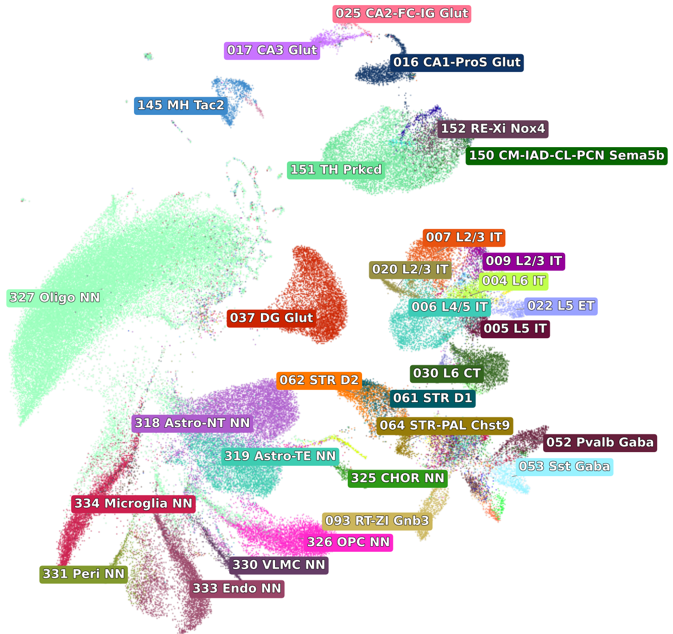
Slide-tags — subclass_name (n = 114,914), top 30 labeled
