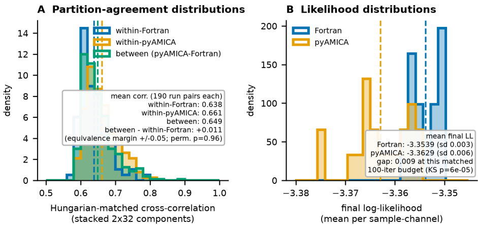
Figure 1: Multi-model solution-ensemble partition-correlation distributions (panel A) and log-likelihood distributions (panel B) for 20 pyAMICA and 20 Fortran fits of the sample EEG; dashed lines mark each distribution's mean. The within-Fortran, within-pyAMICA, and between-implementation correlation distributions overlap, so the single-run correlation reflects the estimator's intrinsic run-to-run spread rather than a gap to the reference. Panel B's apparent separation is a mean log-likelihood gap of only 0.009 on an axis spanning \sim 0.02 .
