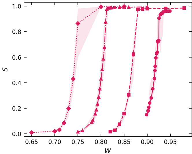
(a) \bullet q=4 \blacksquare q=5 \blacktriangle q=7 \blacklozenge q=10
