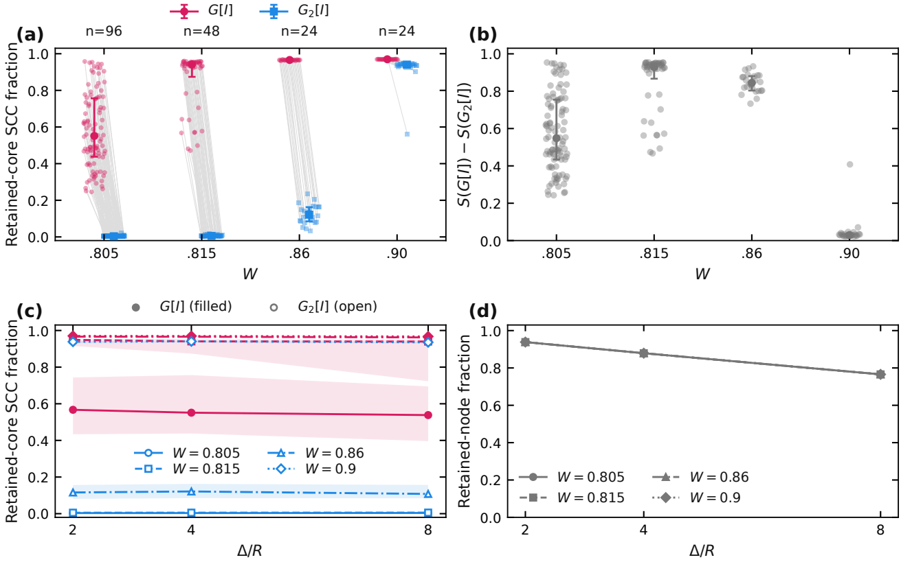
Figure S9: Boundary deletion on all 192 eligible Gaussian L/R = 128 , q = 7 , \sigma R^2 = 24 graphs at W = 0.805, 0.815, 0.86, 0.90 . Counts are 96,48,24,24 at every width. (a) Individual paired full and G_2 SCC fractions after 4R deletion, with median/IQR summaries and faint pair connectors. (b) Corresponding individual paired differences and median/IQR. (c) Width dependence at \Delta/R = 2, 4, 8 : magenta denotes the full graph, blue G_2 , and markers/line styles distinguish W and filled/open markers identify G/G_2 ; bands are IQRs. (d) Retained-node fractions, median/IQR, at the same widths and counts. Original complete-graph labels are restricted by induction; all fractions use the retained node count.
