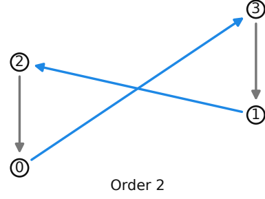
Figure S6: Feedback-order witnesses. (a) Two-vertex order-one toy; green is the upward edge, gray is its downward return. (b) Four-vertex order-two toy; blue upward edges connect gray downward paths. Coordinates are schematic progress coordinates, not a spatial realization.
