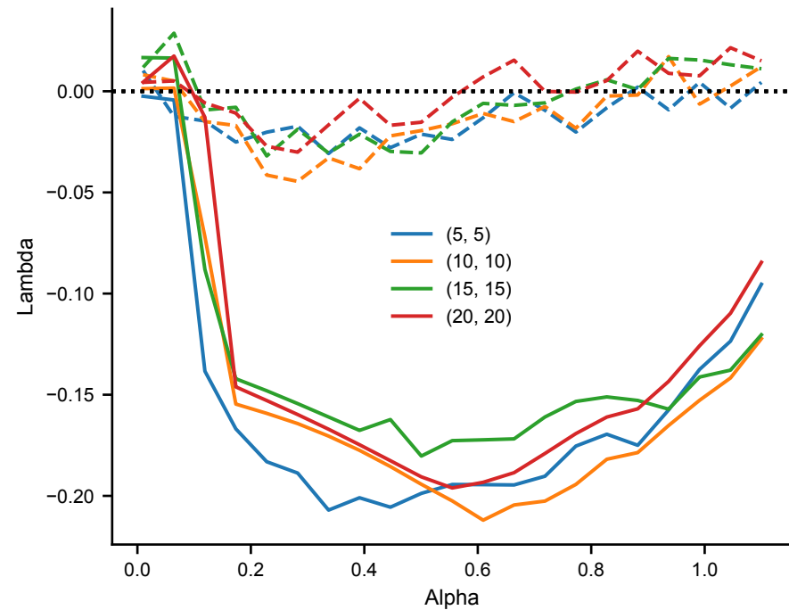
A Largest Lyapunov Exponent
