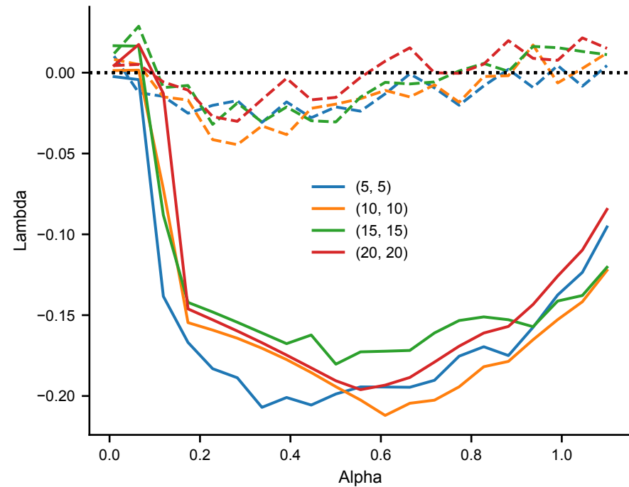
Largest Lyapunov Exponent
