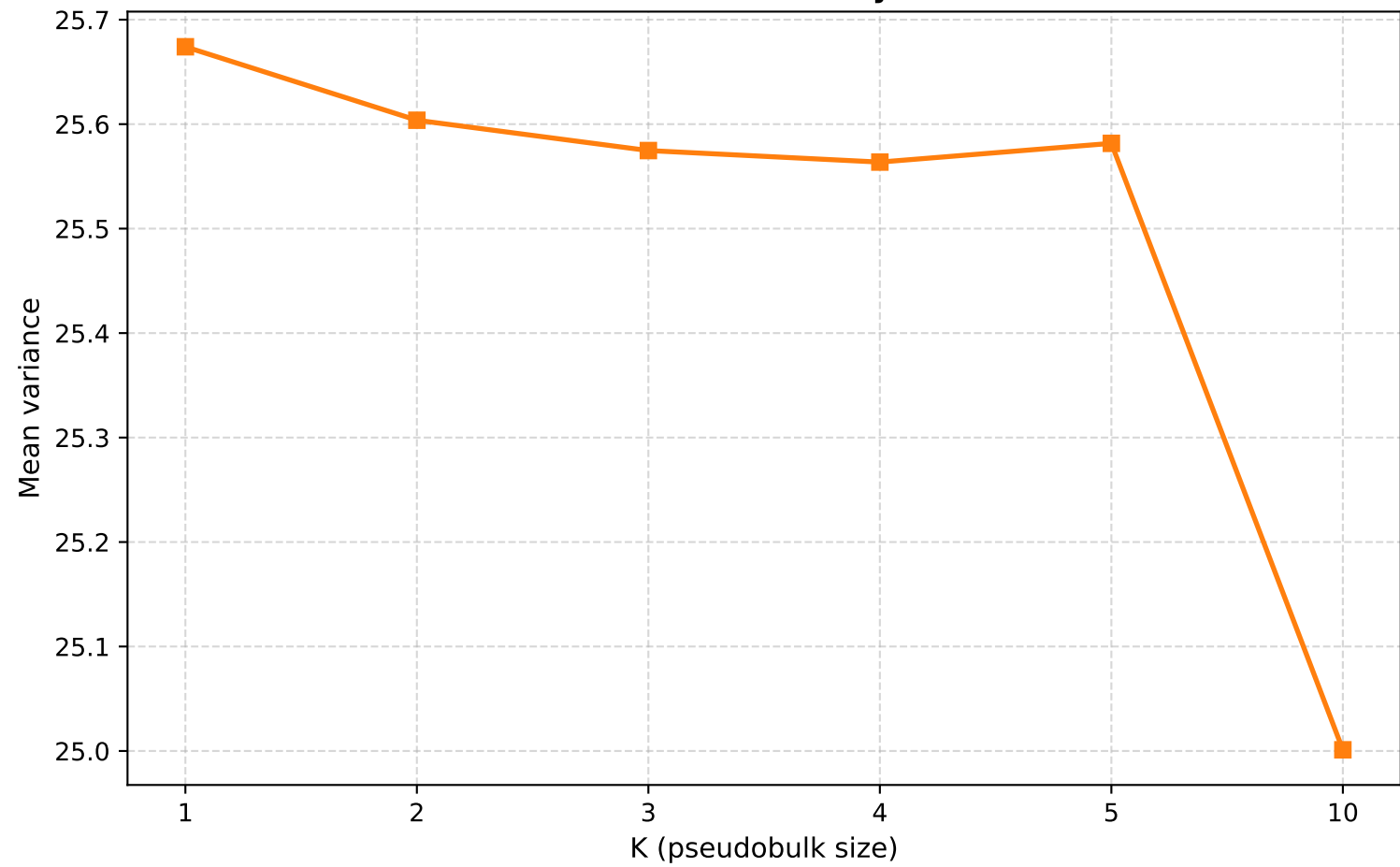
Variance decay
