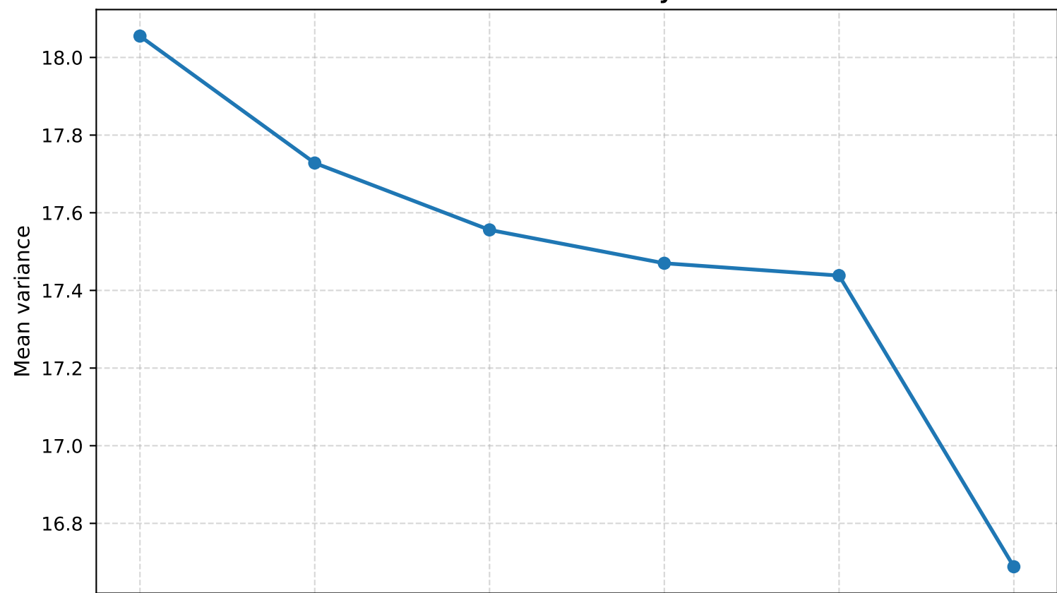
Variance decay
