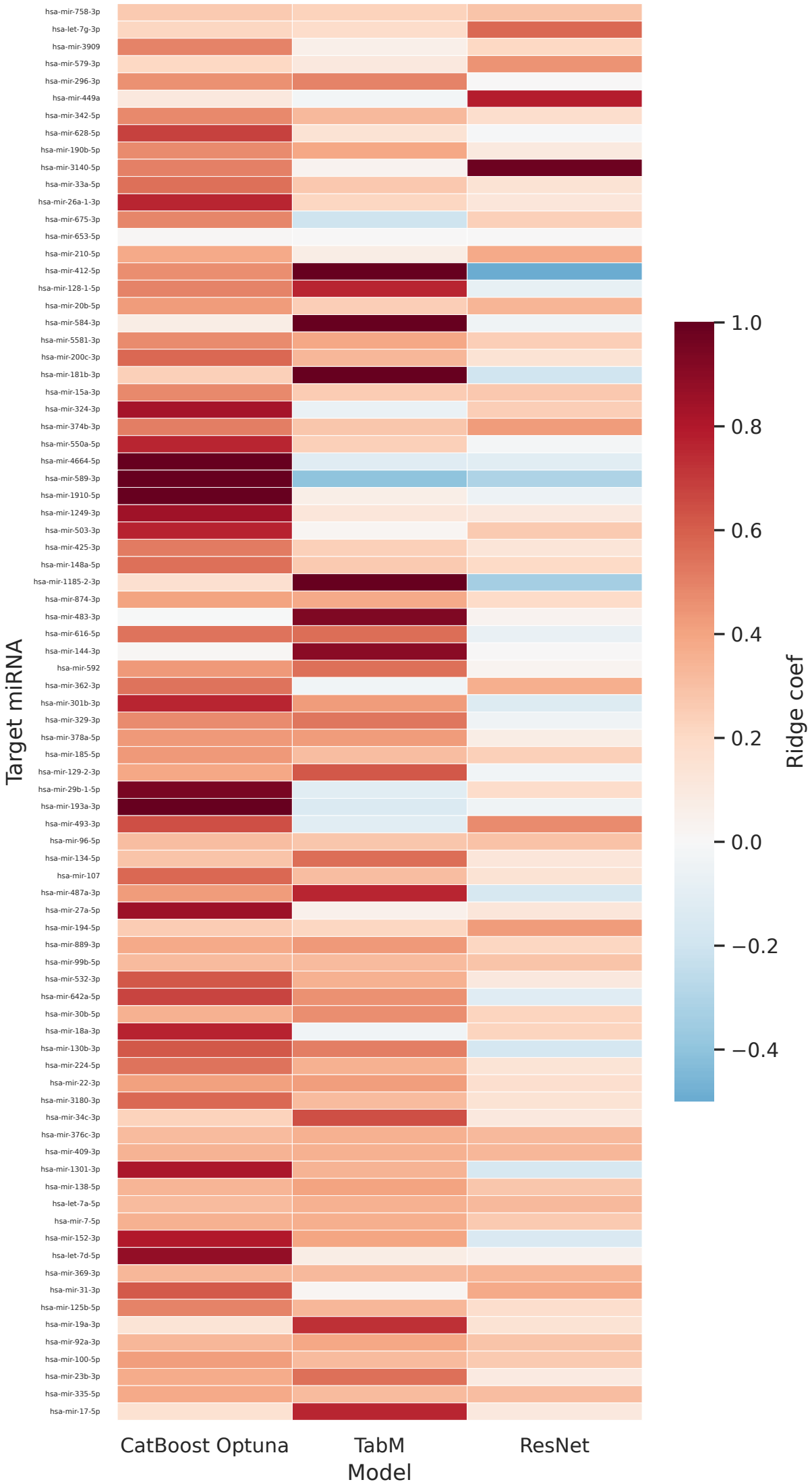
Ridge coefficients by target
