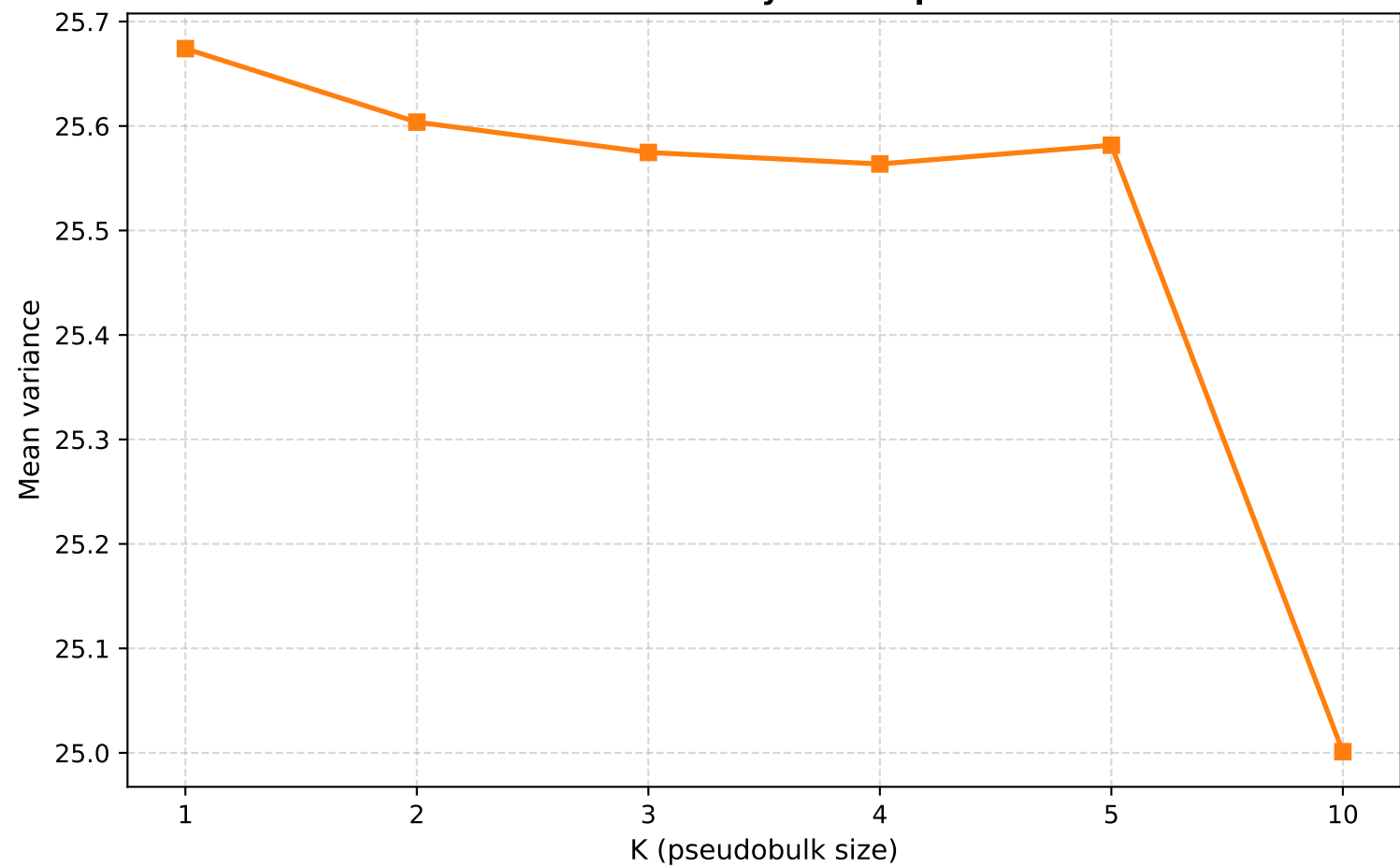
Variance decay miRNA parts
