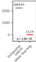
Runtime, hours
