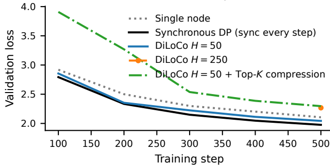
(a) Loss vs. steps
