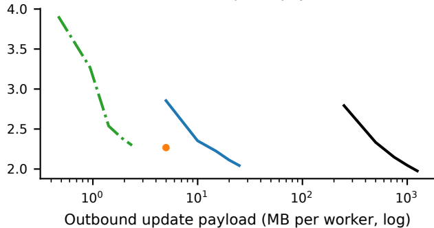
(b) Loss vs. update payload
