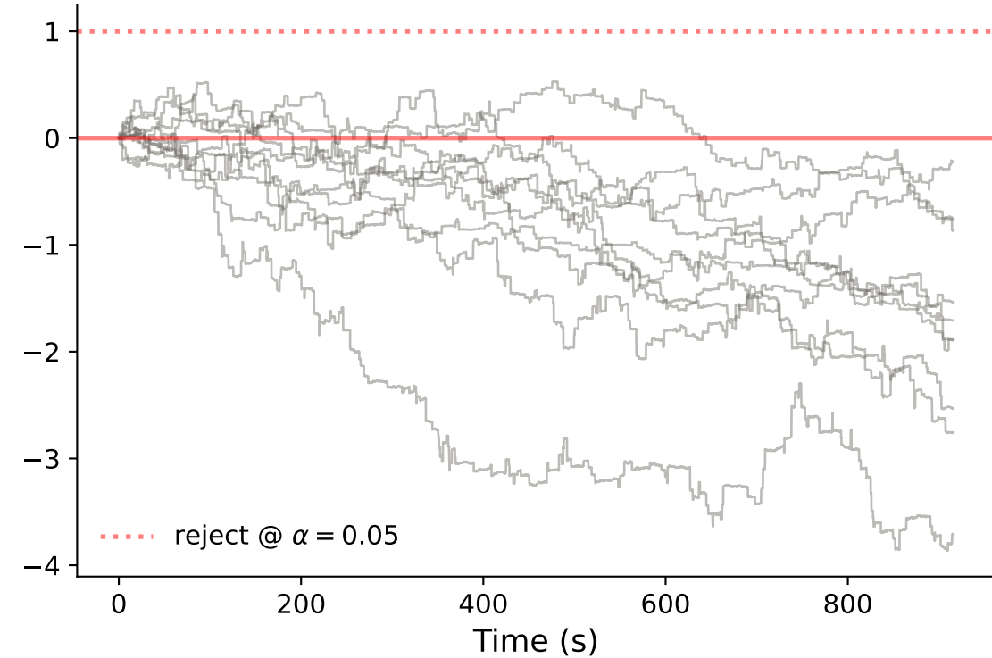
Weak cell 37 -0.002 \alpha -rej/s (0/10 reject)
