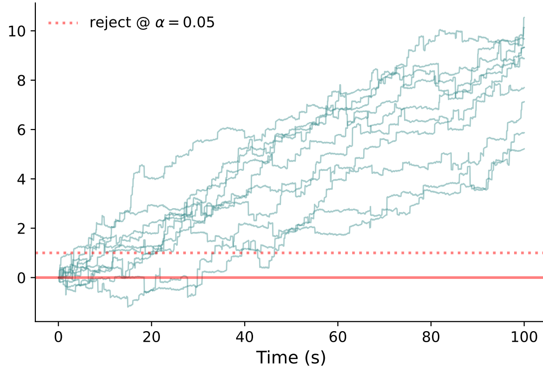
Intermediate cell 8 +0.092 \alpha -rej/s (10/10 reject)
