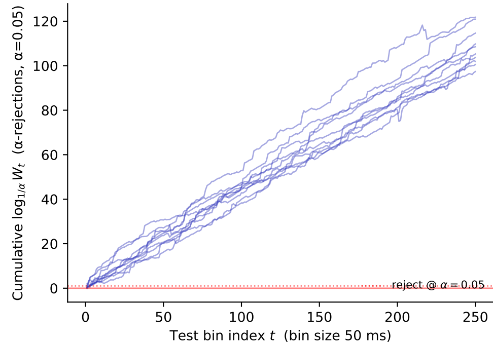
Strong cell 24 +8.526 \alpha -rej/s avg, rejected 10/10
