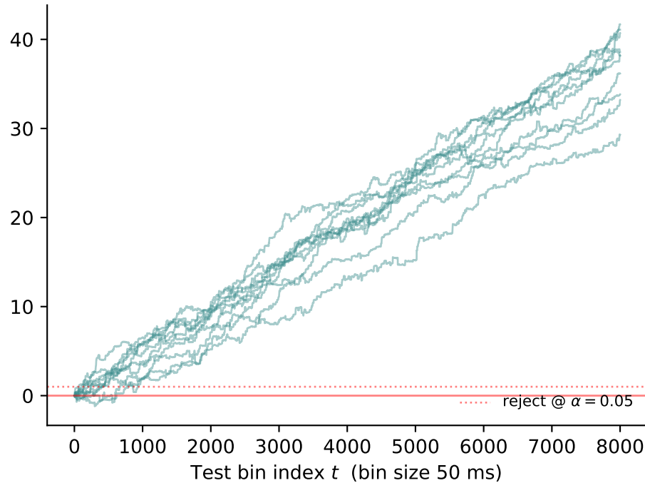
Intermediate cell 8 +0.092 \alpha -rej/s avg, rejected 10/10
