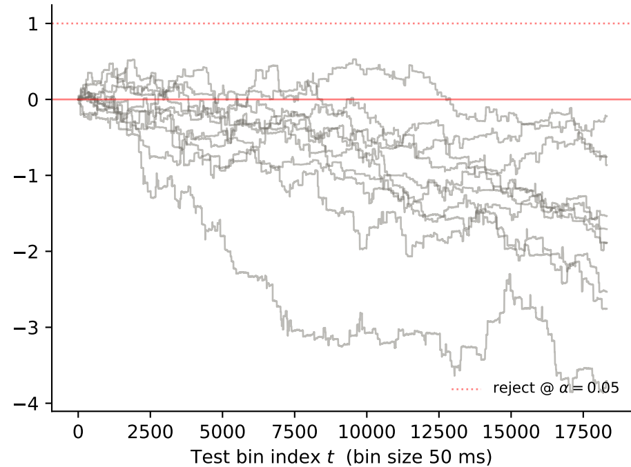
Weak cell 37 -0.002 \alpha -rej/s avg, rejected 0/10
