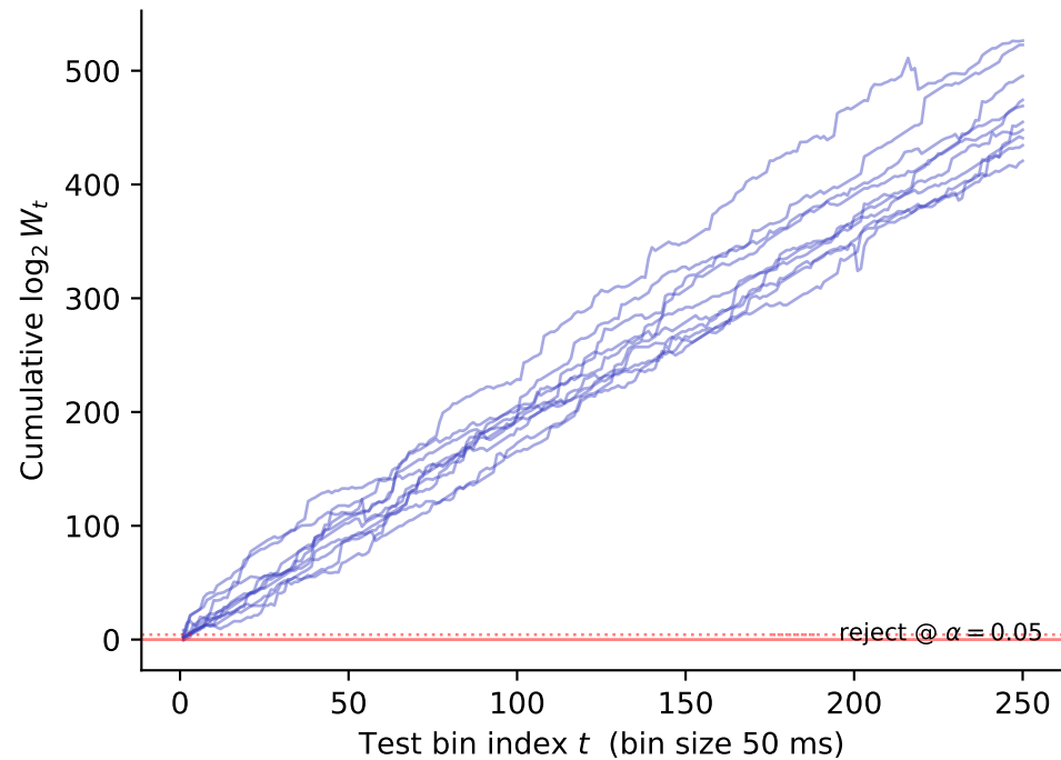
Strong cell 24 +36.848 bits/s avg, rejected 10/10
