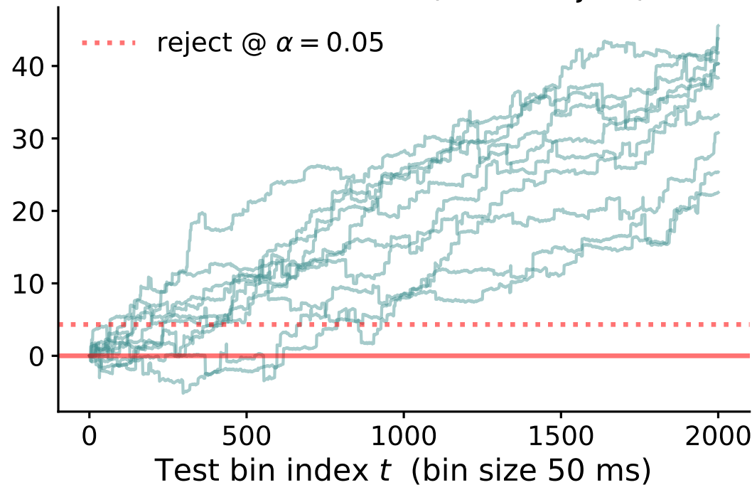
Intermediate cell 8 +0.020 bits/bin (10/10 reject)
