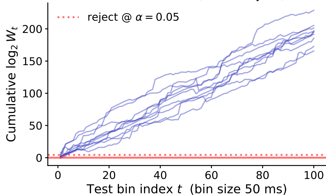
Strong cell 24 +1.842 bits/bin (10/10 reject)
