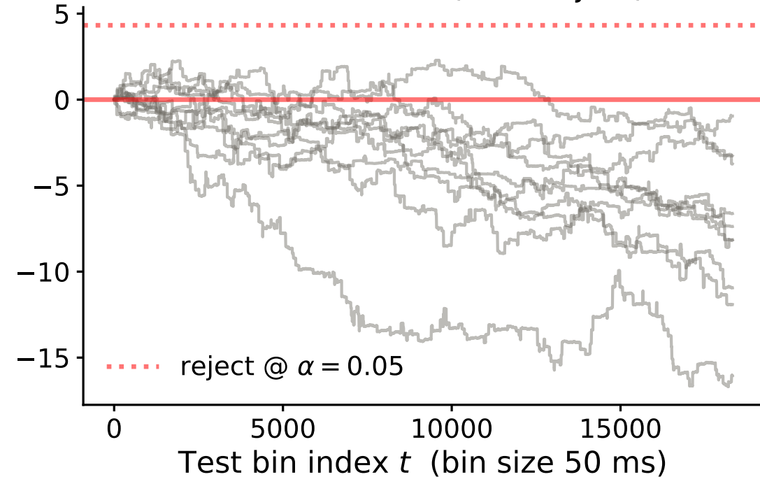
Weak cell 37 -0.000 bits/bin (0/10 reject)
