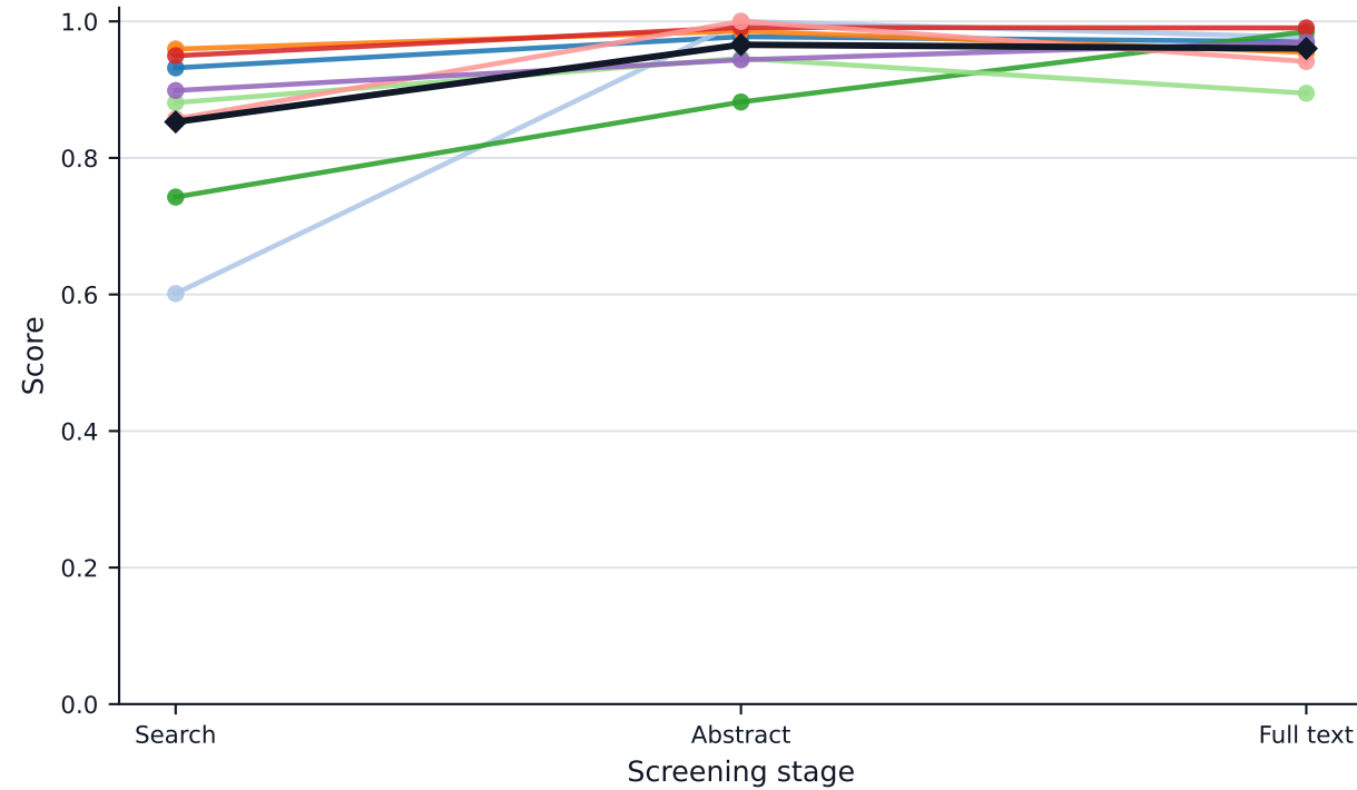
Recall
