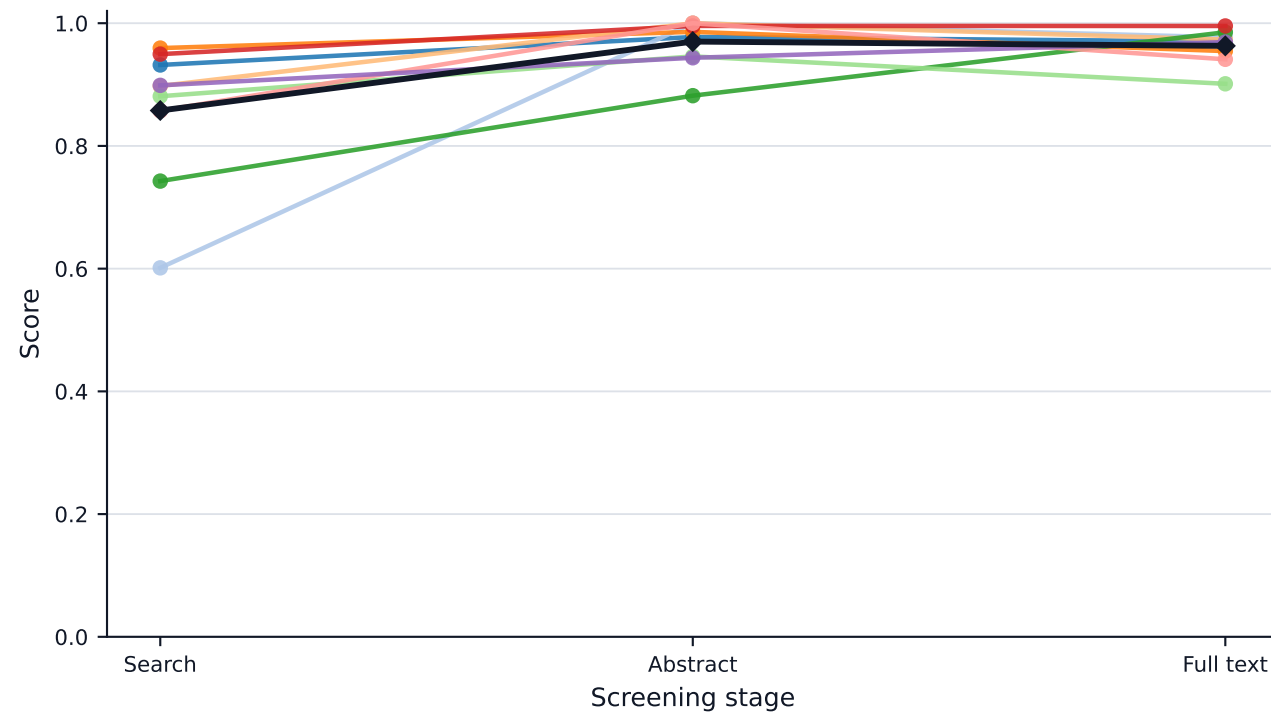
Recall
