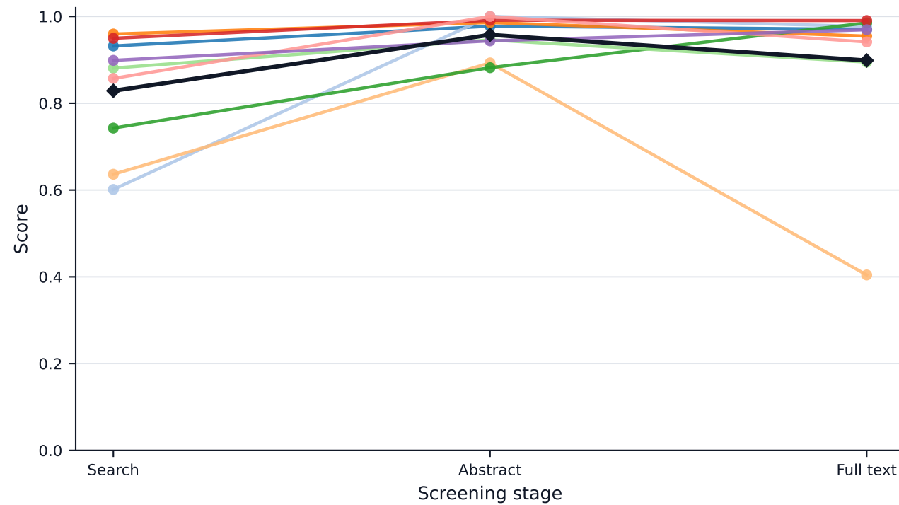
Recall
