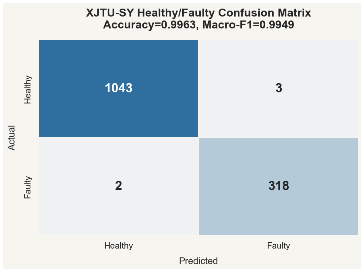
Figure 3: XJTU-SY 混淆矩阵热力图
