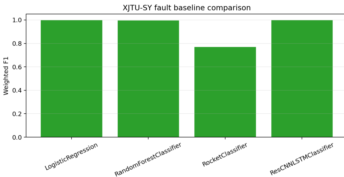
Figure 7: Fault Baseline 对比
