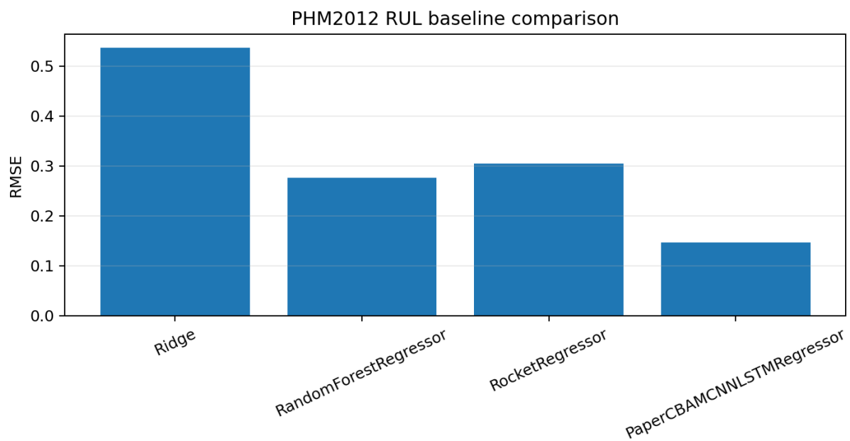
Figure 6: RUL Baseline 对比
