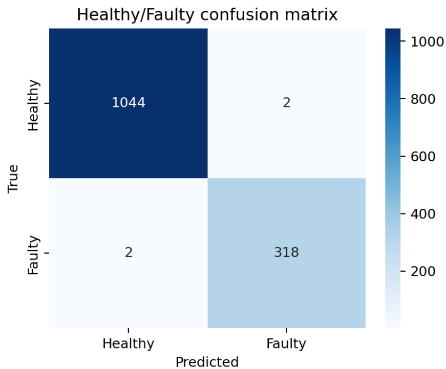
Figure 5: XJTU-SY 混淆矩阵热力图
