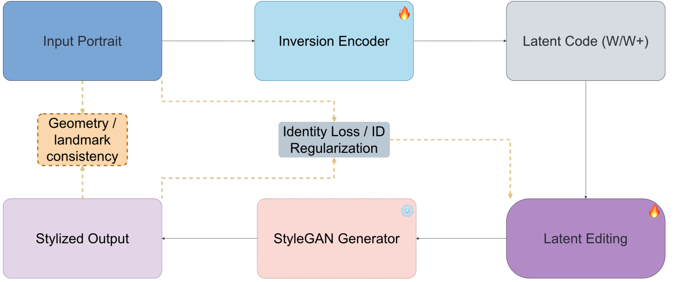
Fig. 2. StyleGAN inversion and latent editing workflow for portrait stylization. The diagram highlights the main forward path and auxiliary identity/geometry regularization branches.
