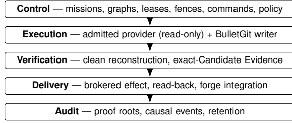
Fig. 1. Five trust planes. A plane may consume only grants addressed to its principal. Portal and any evolutionary optimizer are projections or requestors, never mutation credentials [49].
