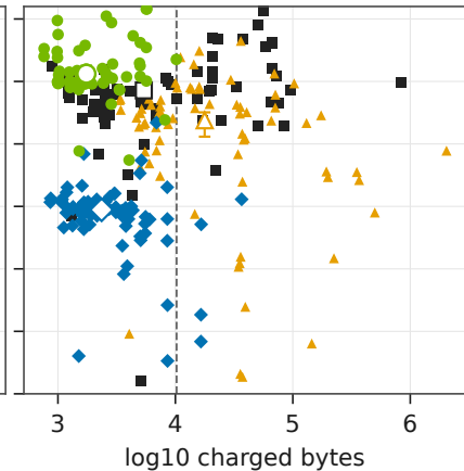
MLP (17 outside)
