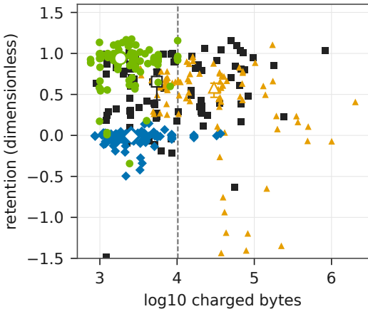
CatBoost (9 outside)
