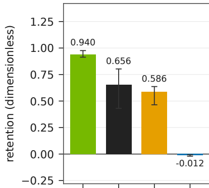
CatBoost, 97 lineages
