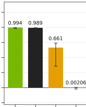
Linear, 92 lineages
