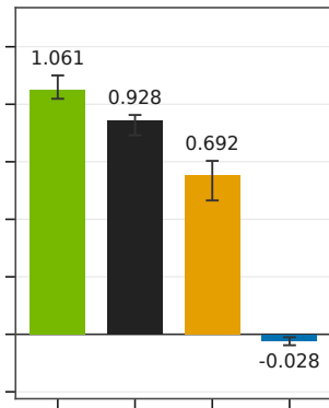
MLP, 75 lineages
