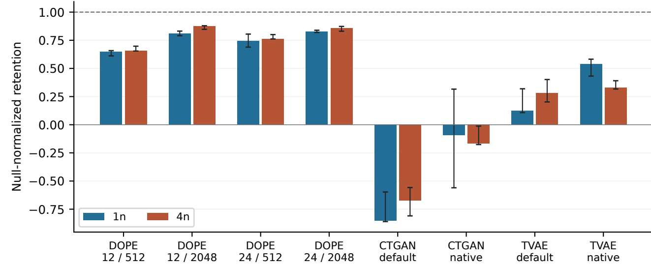
1191_BNG_pbc 0f86a714ec5f3ac6
