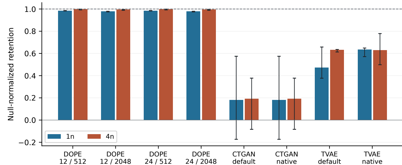
663_rabe_266 a863cd42be4d05d4
