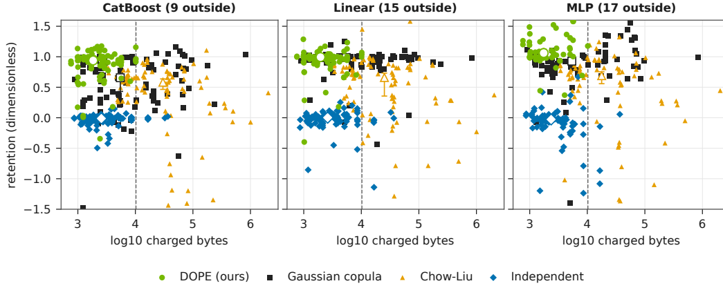
Figure 5: Density-block retention at 4n against charged bytes, per lineage, fit seed 11. Each point is one lineage’s retention level (vertical) against its charged bytes on a log axis. Values outside [-1.5, 1.6] are counted in the panel title and omitted from the frame. The dashed line is the 10,240-byte cap. No Holm family.
