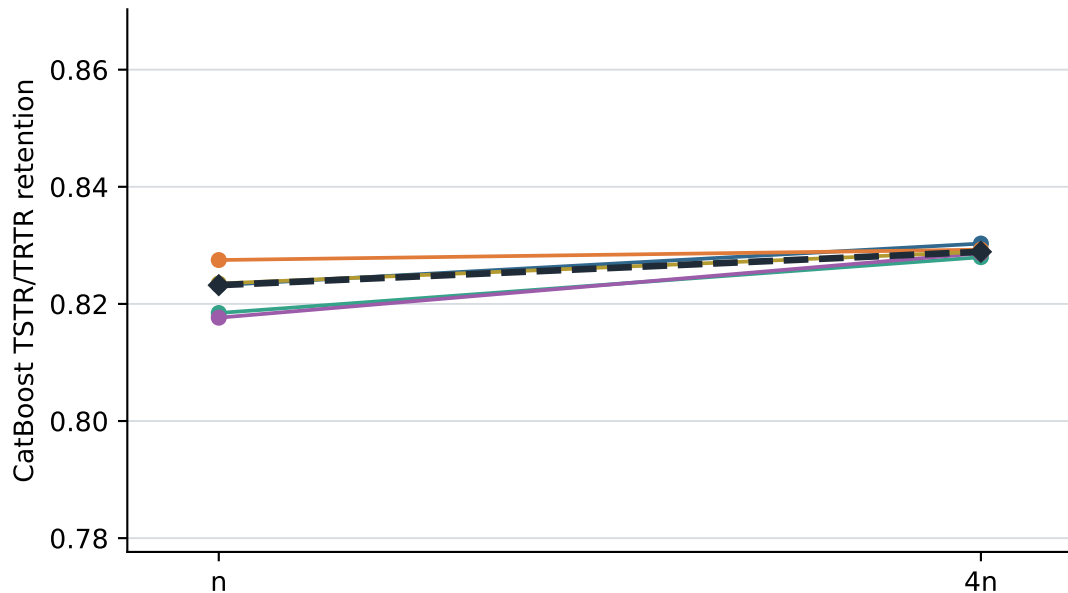
Adult
