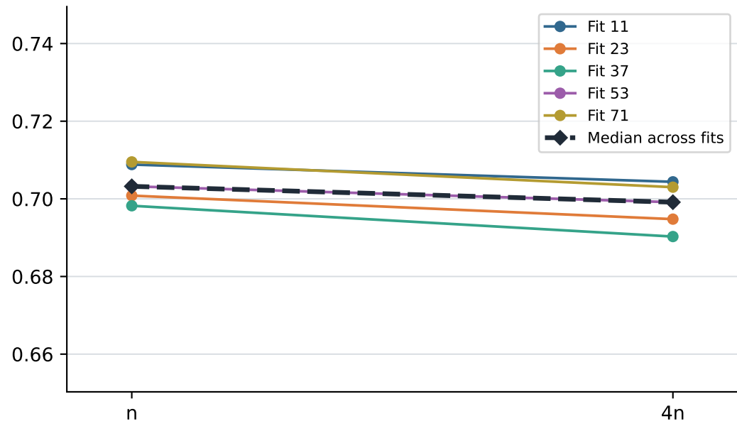
California
