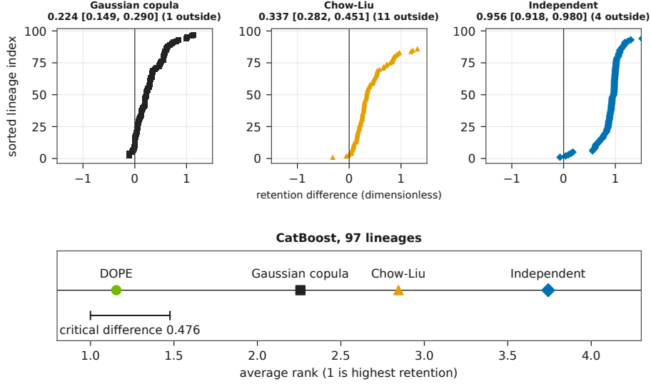
Figure 4: CatBoost paired differences, sorted, and the Nemenyi scale. Rank 1 is the higher retention. The segment length is the critical difference.
