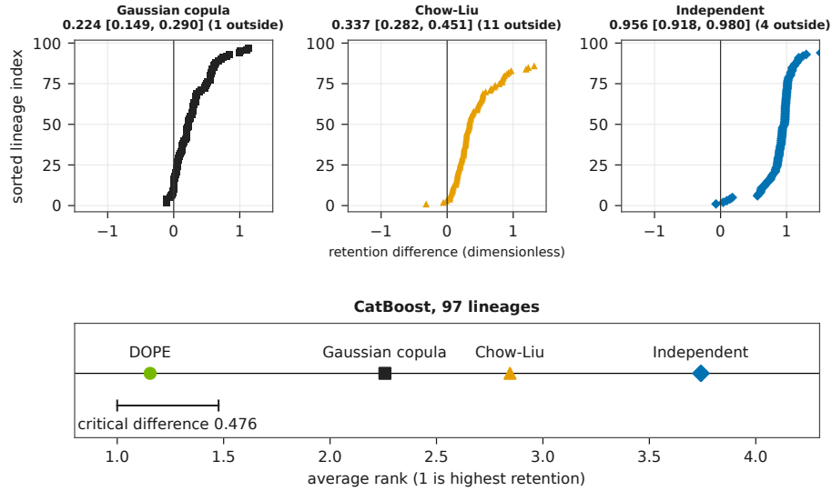
Figure 2: CatBoost paired differences, sorted, and the Nemenyi scale. The denominator is the sorted paired lineages. Rank 1 is the higher retention. The segment length is the critical difference. This display stays outside the nine-test Holm family.
