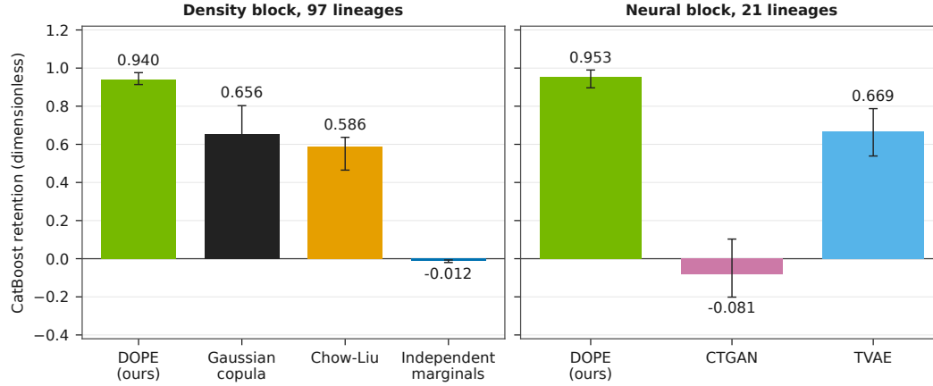
Figure 7: CatBoost retention at 4n. Higher is better. DOPE names the encoding’s generator. Each bar is a method’s paired-lineage retention median and its lineage-bootstrap interval. Density uses 97 lineages. The neural panel uses 21 and stays unpooled. Forest-Flow, 6 lineages, is higher on its own block and is omitted. No Holm family is drawn. The tests are in the tables.
