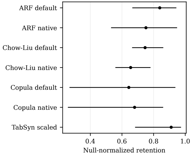
Matched eight, 4n; 95% lineage CI
