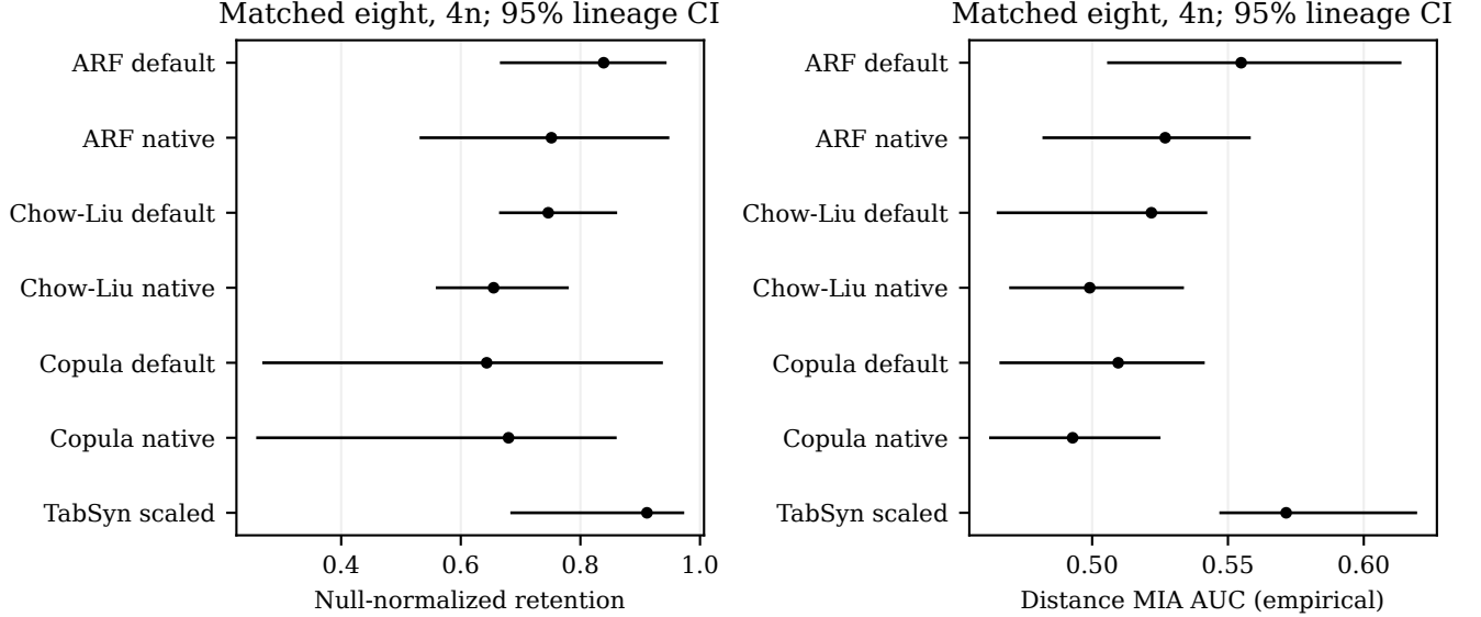
Fig. 5. Matched retained subset: median and marginal lineage-bootstrap intervals. Privacy AUC is an empirical diagnostic; its interval is not a privacy guarantee.
