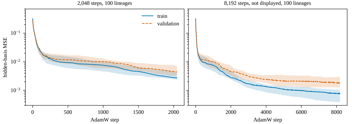
Fig. 1. Logged replay of both step budgets before the readout refit. The solid line is the training median and the dashed line is the validation median. Each band is a 95% lineage-bootstrap interval. The longer budget is not the displayed model.
