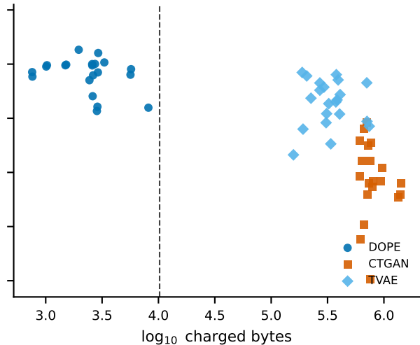
Neural block, shared 21 lineages
