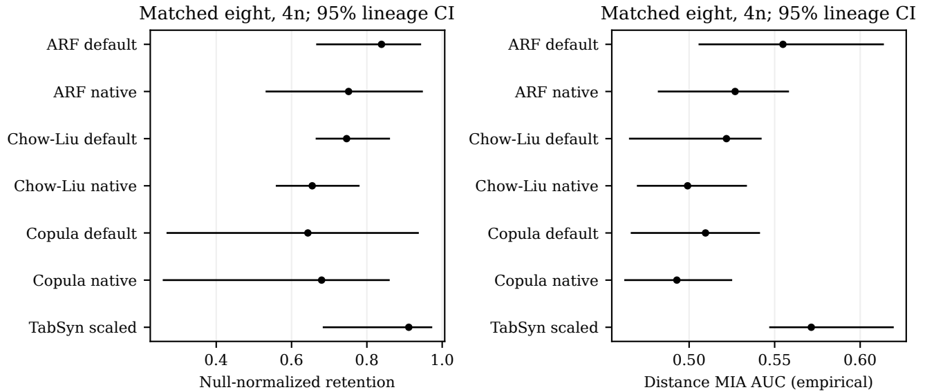
Fig. 7. Matched retained subset: median and marginal lineage-bootstrap intervals. Privacy AUC is an empirical diagnostic; its interval is not a privacy guarantee.
