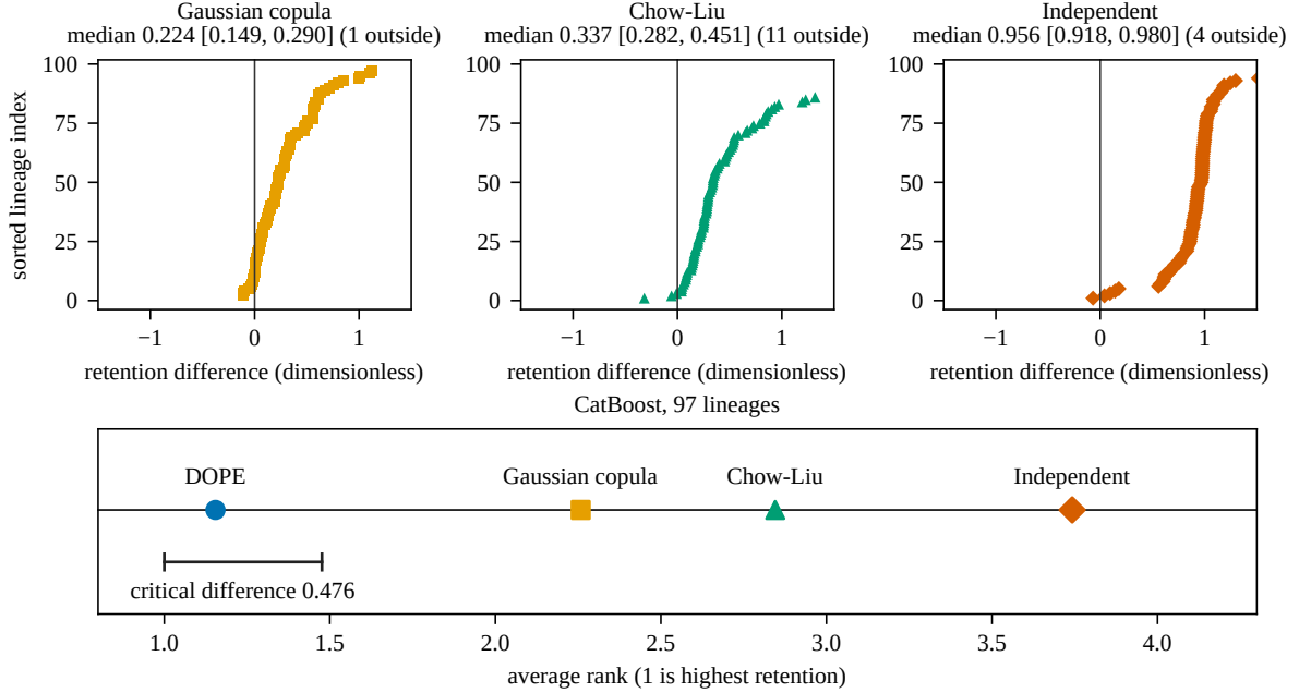
Fig. 4. CatBoost paired differences, sorted, and the Nemenyi scale. Rank 1 is the higher retention. The segment length is the critical difference.
