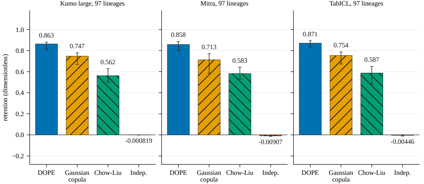
Fig. 5. Kumo large, Mitra, and TabICL retention at 4n . Higher is better. Each bar is the lineage median and its lineage-bootstrap interval. Hatches distinguish the methods. This panel is not an MFS value.
