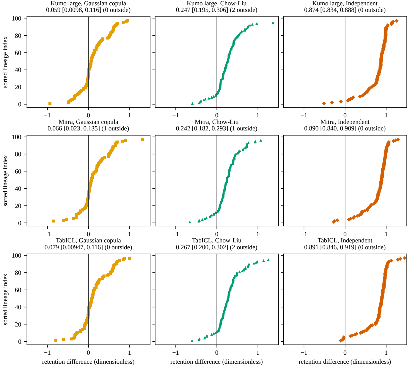
Fig. 6. Paired retention differences for Kumo large, Mitra, and TabICL, sorted by lineage. Filled marks are lineages.
