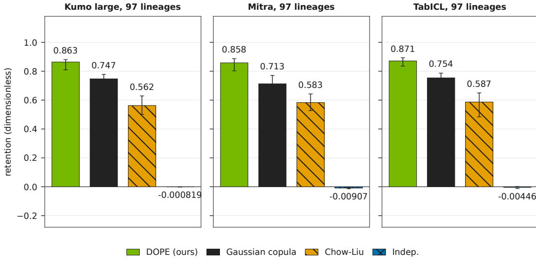
Figure 3: Kumo large, Mitra, and TabICL retention at 4n . Higher is better. Each bar is the lineage median and its lineage-bootstrap interval. The denominator is the paired informative lineages in that panel. Hatches distinguish the methods. Holm family size is three per auditor and is reported in the main paper. This panel stays outside MFS.
