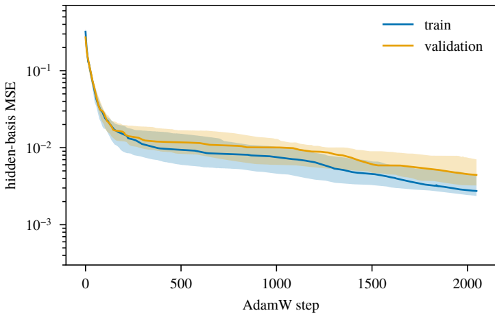
2,048 steps, 100 lineages
