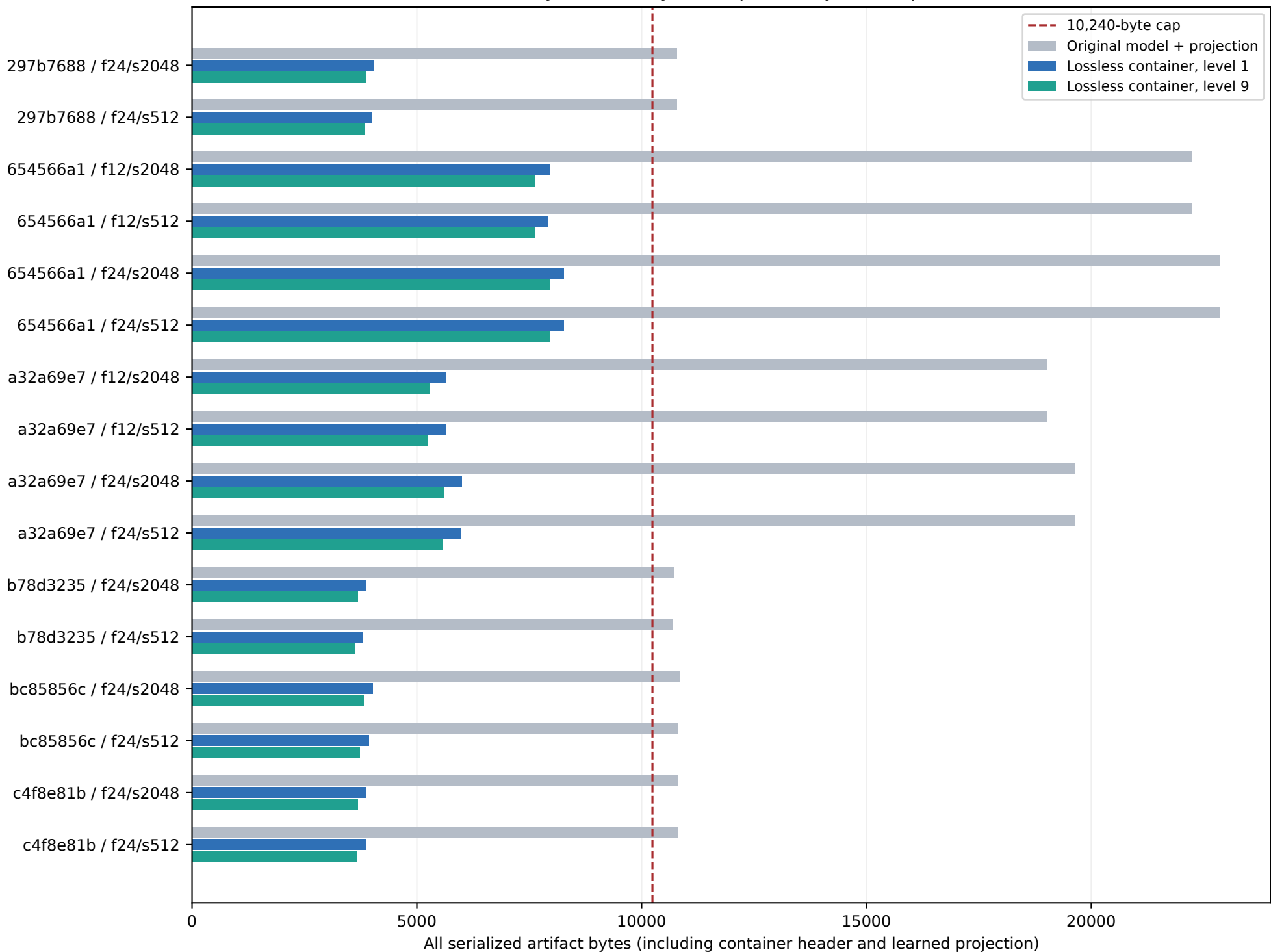
Lossless byte feasibility for 16 previously over-cap DOPE fits
