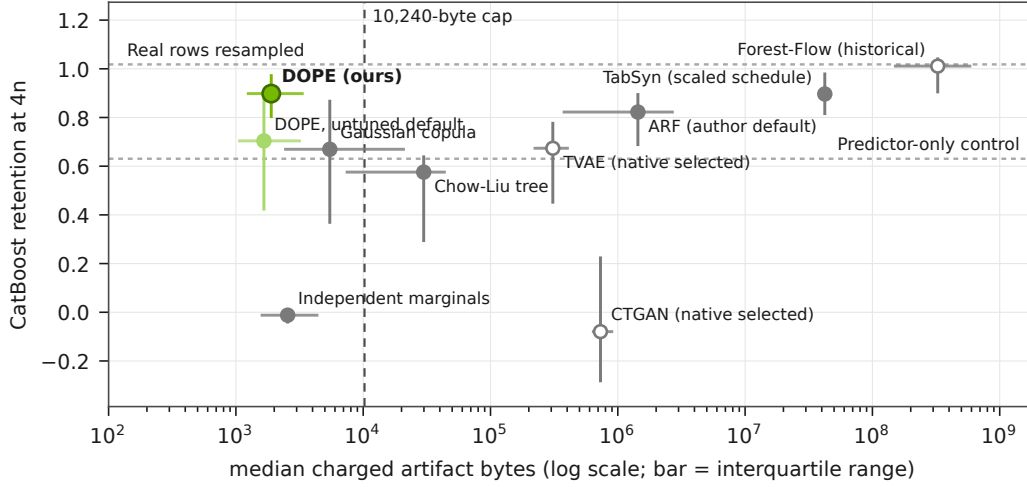
Figure 2: CatBoost retention at 4n against median charged artifact bytes. Points are lineage medians with 95% nested bootstrap intervals (vertical) and the interquartile range of bytes (horizontal). Hollow points are cohorts below 90 lineages. The light green point is DOPE’s untuned default. Horizontal lines are the two controls, which store no artifact. The dashed line is the 10,240-byte release cap. Byte medians use each method’s lineages with a charged fit, counted in Table 1; points come from unpaired cohorts, and Table 1 gives the paired comparison. No Holm family.
