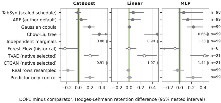
Figure 1: DOPE minus the main comparators and both controls at synthetic size 4n . Hodges–Lehmann paired retention difference with its 95% nested bootstrap interval; the vertical line marks zero, and Table 1 adds native-selected ARF and the untuned default. Open marks are cohorts below 90 lineages, grey marks are controls, and the number beside a row is its CatBoost paired lineage count. The band is the equivalence margin \pm 0.02 ; the axis runs from -0.3 to 0.5 , with an edge arrow and its value for any difference beyond it. Holm families are in Table 1.
