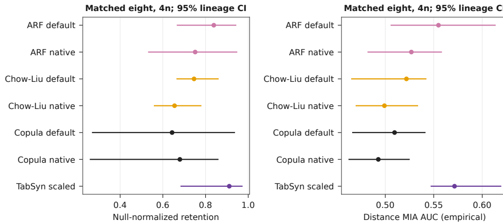
Figure 8: Earlier eight-lineage TabSyn subset: medians and marginal lineage-bootstrap intervals. No Holm family. Privacy AUC is an empirical diagnostic.
