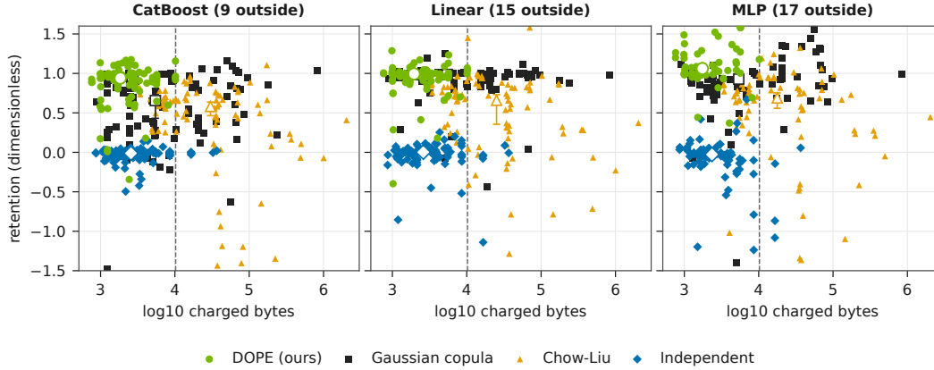
Figure 5: Density-block retention at 4n against charged bytes, per lineage, fit seed 11. Each point is one lineage’s retention level (vertical) against its charged bytes on a log axis. Values outside [-1.5, 1.6] are counted in the panel title and omitted from the frame. The dashed line is the 10,240-byte cap. No Holm family.
