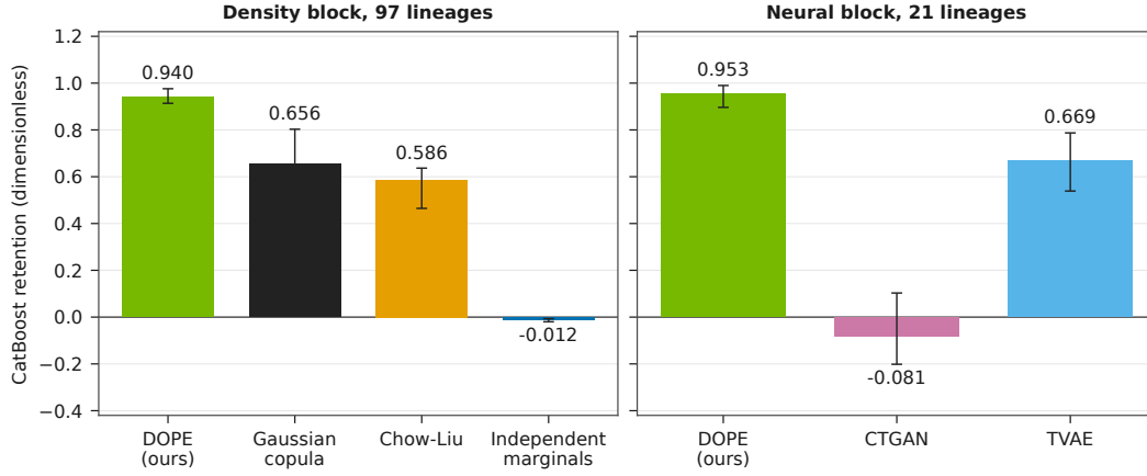
Figure 4: CatBoost retention at 4n , fit seed 11. Each bar is a method’s paired-lineage retention median and its lineage-bootstrap interval. Density uses 97 lineages and the neural panel 21; the panels are separate cohorts. No Holm family.
