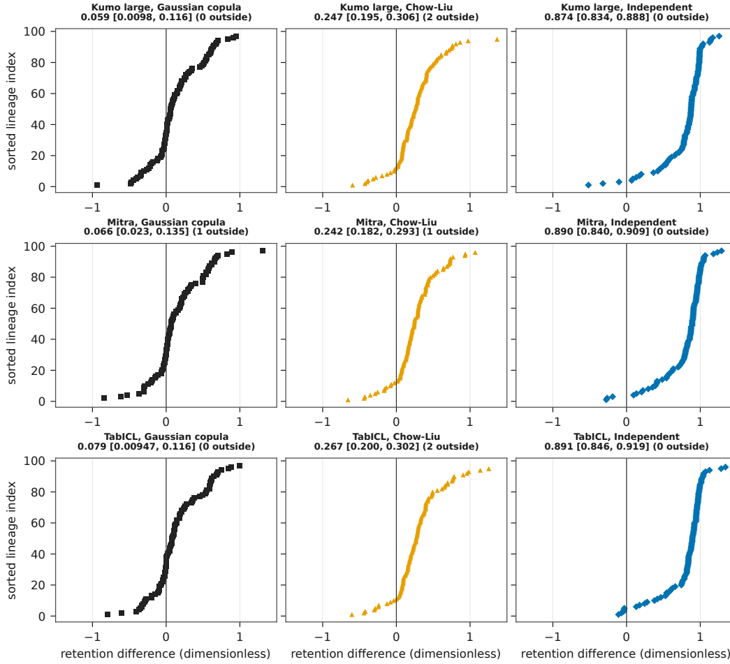
Figure 3: Paired retention differences for Kumo large, Mitra, and TabICL, sorted by lineage. The denominator is the paired informative lineages in that panel. Holm family size is three per auditor.
