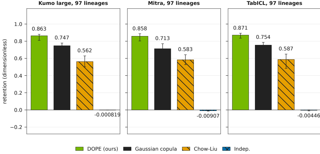
Figure 2: Kumo large, Mitra, and TabICL retention at 4n . Each bar is the lineage median and its lineage-bootstrap interval; the denominator is the paired informative lineages in that panel. Holm family size is three per auditor.
