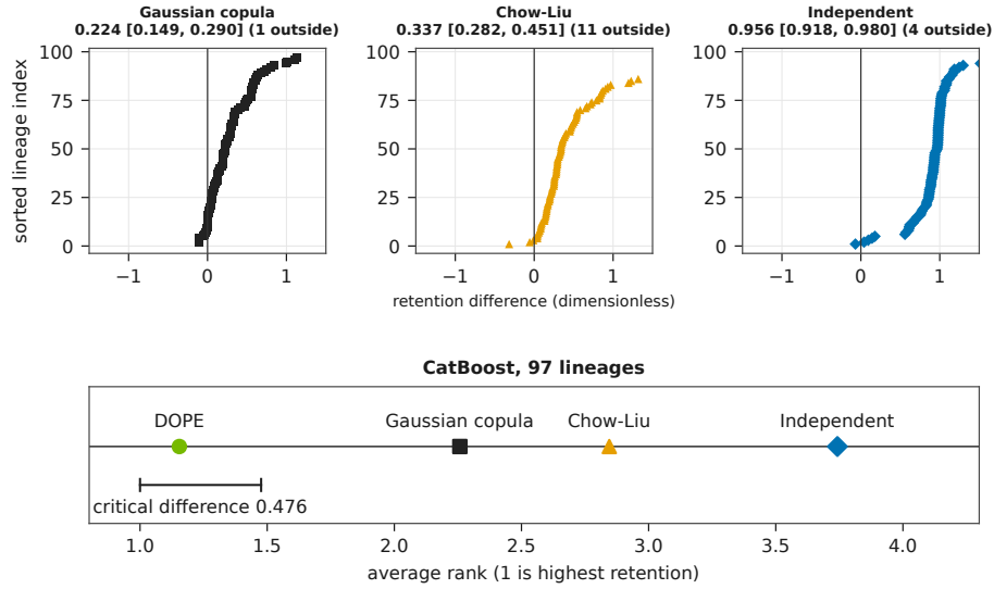
Figure 6: CatBoost paired differences, sorted, and the Nemenyi scale, fit seed 11. Rank 1 is the higher retention; the segment length is the critical difference. This display is outside the nine-test Holm family.
