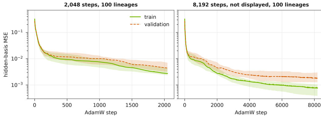
Figure 7: Logged replay of both step budgets before the readout refit. The solid line is the training median and the dashed line the validation median; each band is a 95% lineage-bootstrap interval. The longer budget is not the reported model.
