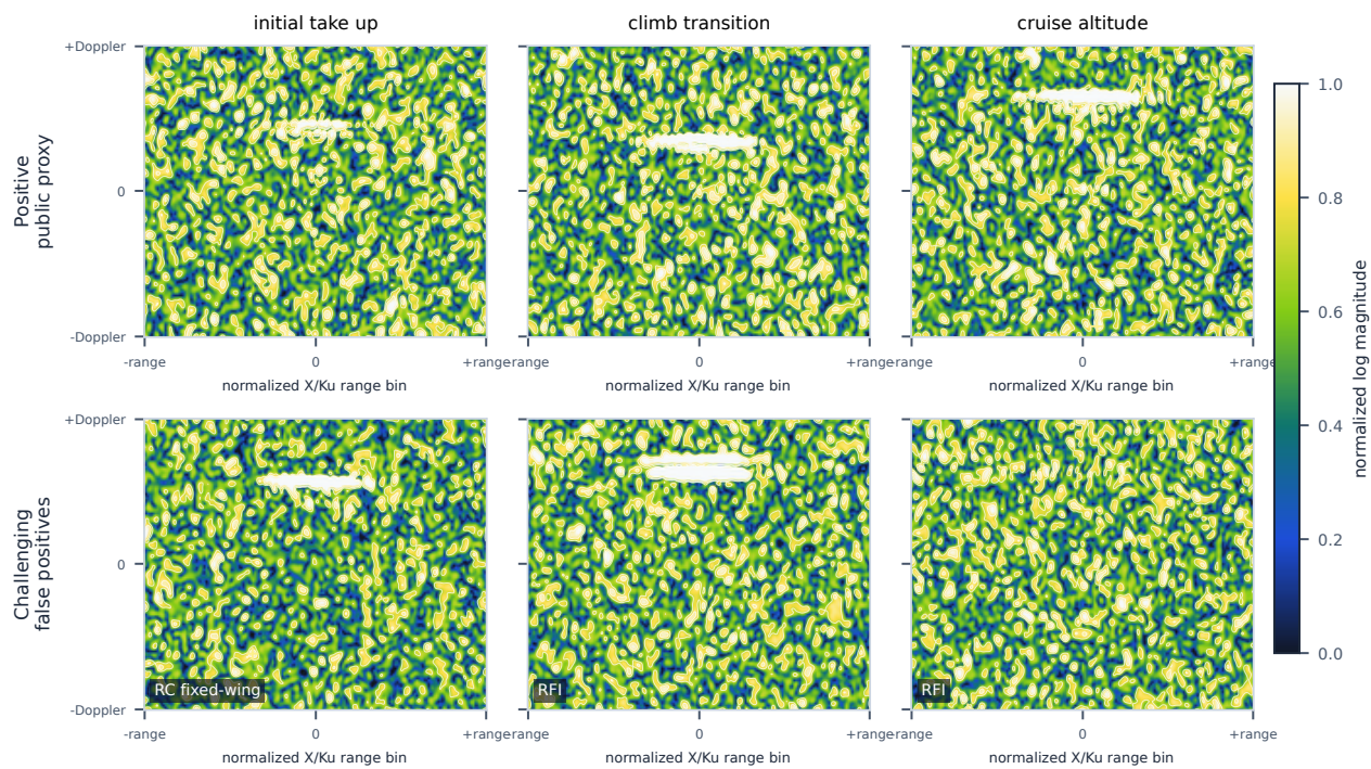
Fig. 5. Range-Doppler diagnostic gallery: fixed-wing pusher-prop public-proxy positives versus challenging EW/clutter false positives. Axes are normalized range-Doppler bins and color is normalized log magnitude after a windowed zero-padded FFT display transform from 64 by 96 X/Ku IQ. These panels are qualitative diagnostics only, not measured imagery and not detector input for the KPI.
