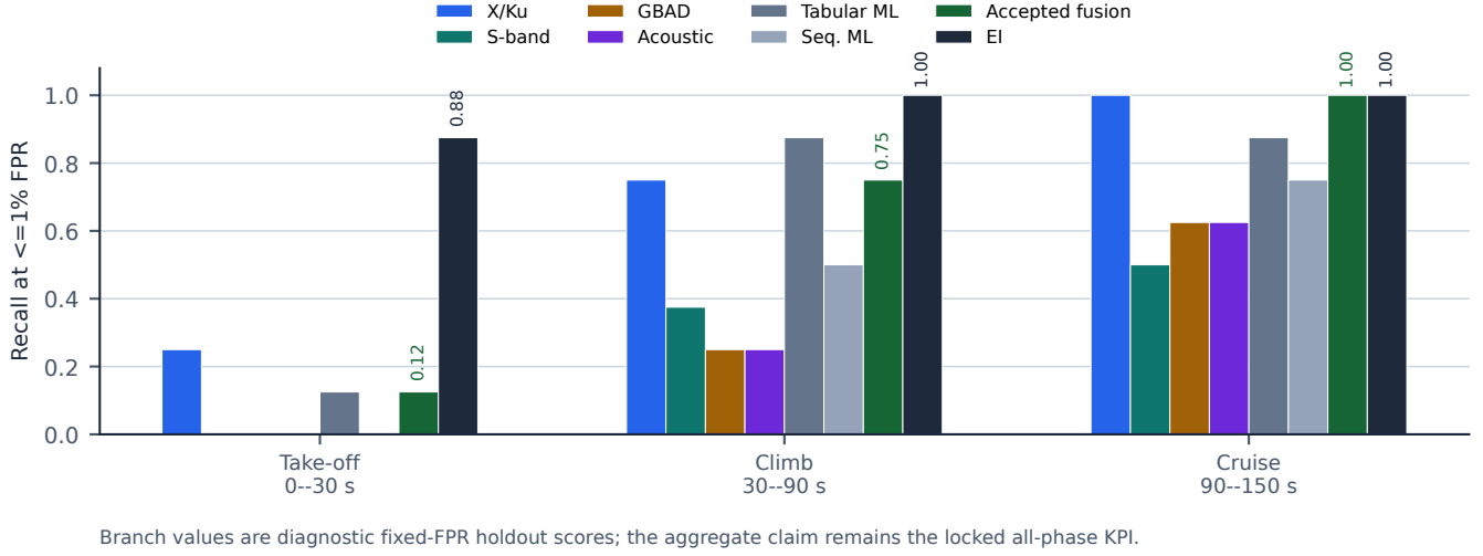
Fig. 2. Human detection ladder and EI challenger by phase. The same take-off, climb, and cruise panels show progression from radar and cue branches to ordinary ML controls, accepted human fusion, and EI. The plotted diagnostic is Recall@ \leq 1\% FPR on the holdout phase slice; phase conclusions remain diagnostic because each phase has only eight positive holdout records.
