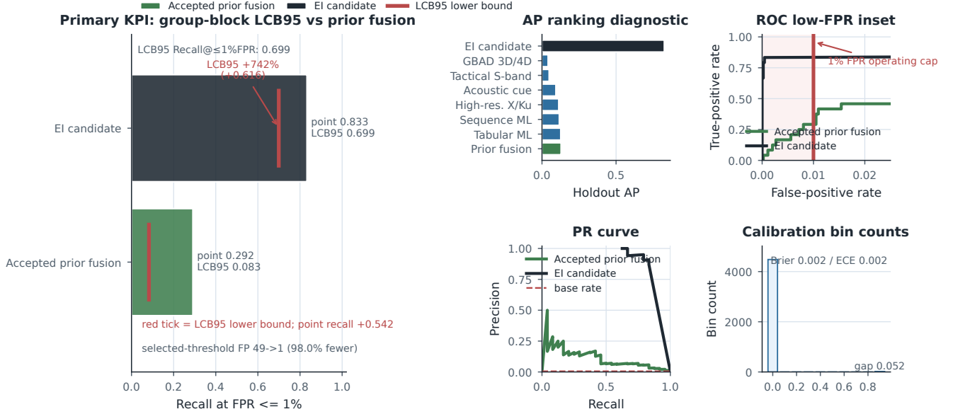
Fig. 4. Holdout primary KPI, ranking diagnostics, low-FPR ROC/PR behavior, and calibration. Red vertical ticks are group-block LCB95 lower bounds, and the pale red shaded zone with the thick red line marks the 1% FPR operating cap. Recall@ \leq 1\% FPR and its LCB95 are the headline quantities; AP, ROC AUC, PR shape, and calibration bins are supporting diagnostics.
