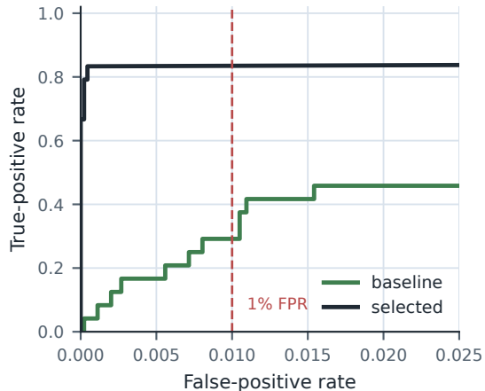
ROC low-FPR inset
