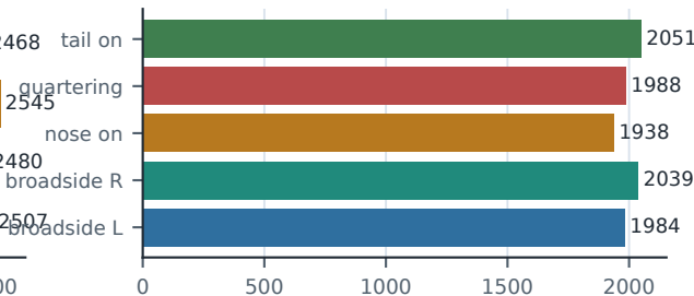
Hard-negative
