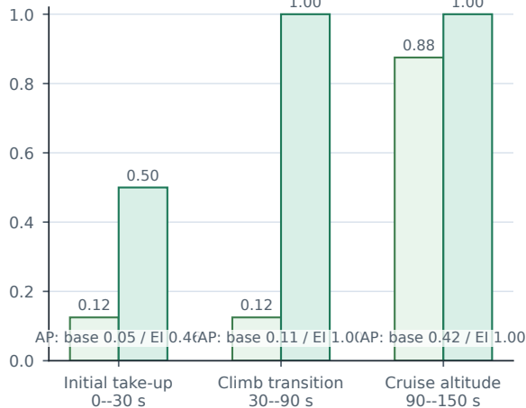
Fixed-FPR recall by phase
