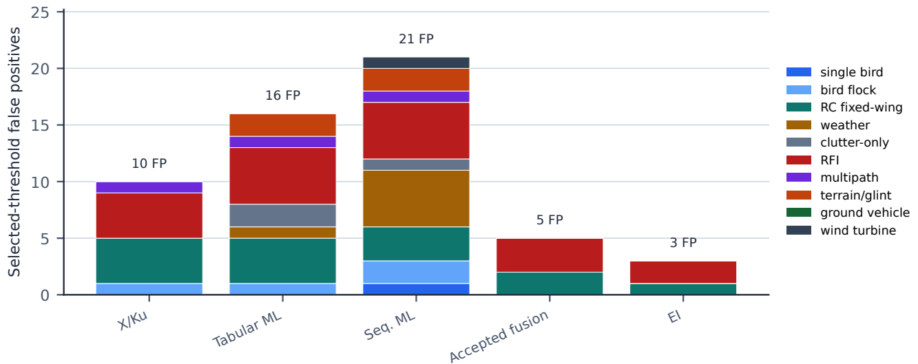
Fig. 4. Selected-threshold false-positive burden by method and hard-negative family. Bird includes single-bird and flock-like confusers; RC fixed-wing includes small model aircraft with prop-cadence overlap; weather includes rain, dust, and weather-cell stress; clutter-only includes no-target scene clutter; RFI includes burst contamination and passive-RF artifacts; multipath includes ghost/reflection-like tracks; terrain/glnt includes site reflections; ground vehicle includes low-altitude track-like vehicle confusers; wind turbine is a rotating-structure hard negative. Near-threshold negatives are retained as evidence guardrails rather than stacked as false positives.
