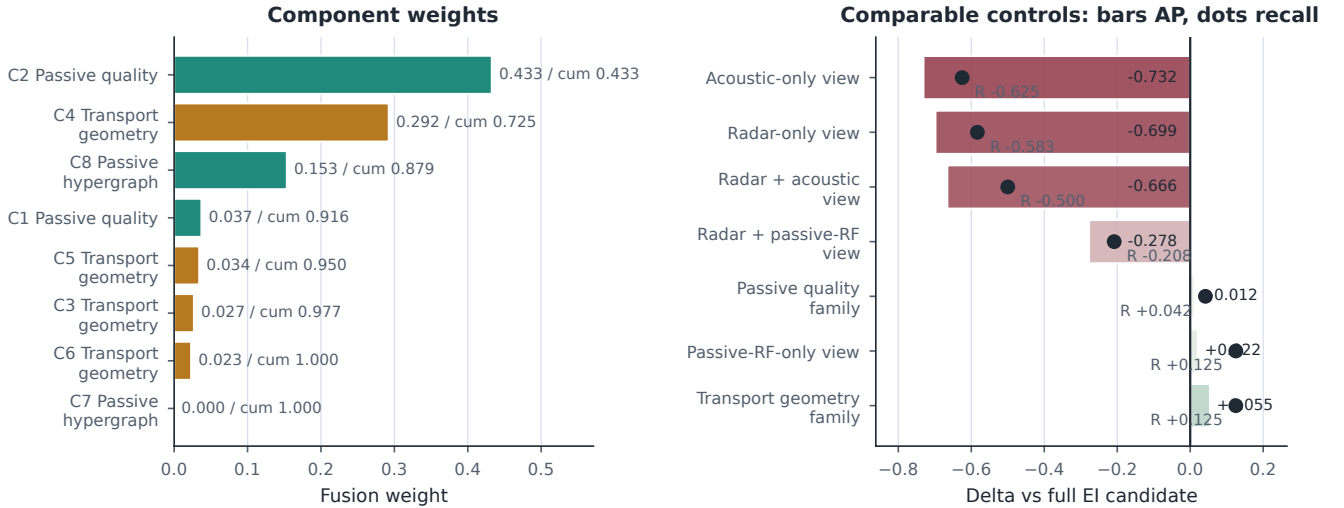
Fig. 6. EI component weights and comparable holdout controls. The left panel sorts human-readable component weights; the right panel reports AP and fixed-FPR recall deltas computed with the same holdout metric definitions as Table VI. Raw component handles and ablation-internal diagnostics remain in evidence artifacts.
