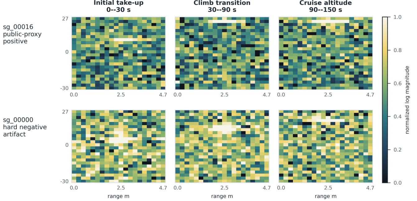
Fig. 8. Range-Doppler proxy diagnostics for a positive public-proxy group and a hard-negative group. Axes show relative range in meters and velocity-equivalent Doppler bins using the X/Ku branch resolution; color is normalized log-magnitude on a shared scale.
