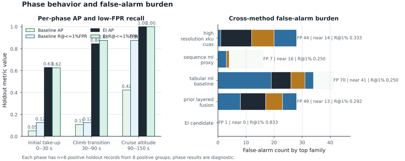
Fig. 4. Per-phase behavior and cross-method false-positive burden. The left panel compares phase-wise AP and fixed-FPR recall for the baseline and EI candidate; the right panel sorts false alarms by family for the strongest methods together with near-threshold context. Each phase has only eight positive holdout records from eight positive groups, so phase conclusions are diagnostic.
