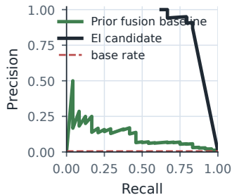
PR curve
