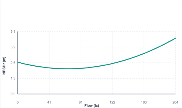
NPSHr vs Flow
