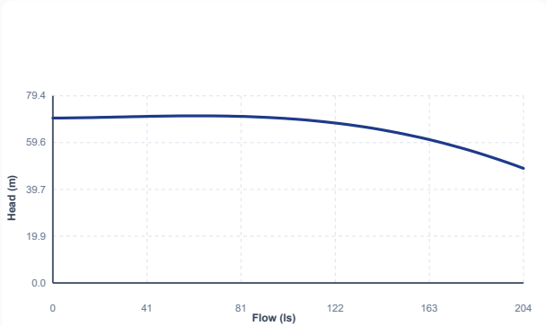
Head vs Flow (H-Q)
