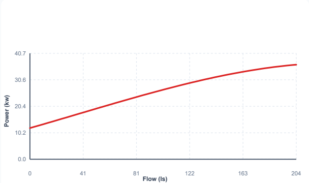
Power vs Flow (P-Q)
