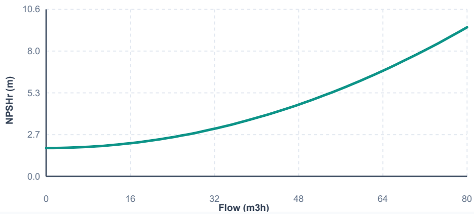
NPSHr vs Flow
