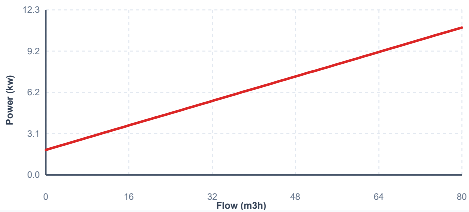
Power vs Flow (P-Q)
